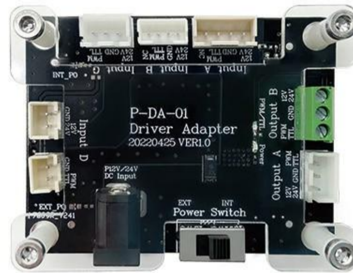
Driver adapter
